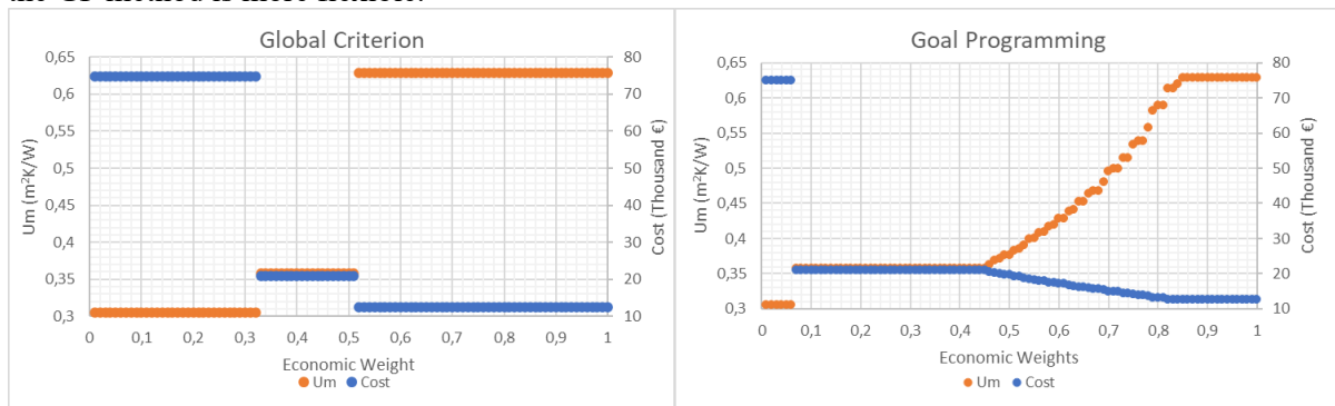
Figure 4. Optimum distribution of Costs and U_m -values in BLC-Cost optimization with Global Criterion and Goal Programming methods.
