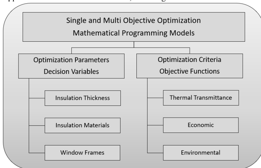
Figure 1. The proposed optimization concept of building envelope energy efficiency improvement.
