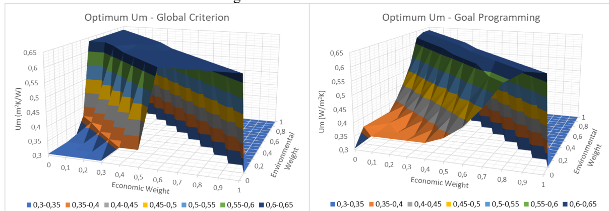
Figure 3. Optimum distribution of U_m -values with Global Criterion and Goal Programming methods.
